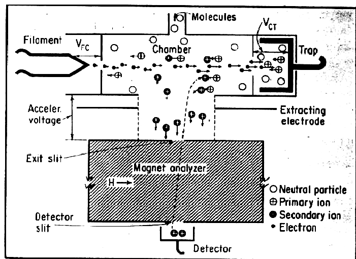
FIG. 1. MASS SPECTRUM ANALYSIS of secondary ions created in charge-transfer collisions with monoatomic primary ions. Voltages in ion source of conventional mass spectrometer are adjusted so that primary ions are created only in region of trap and charge-transfer reactions occur in ion source chamber.
